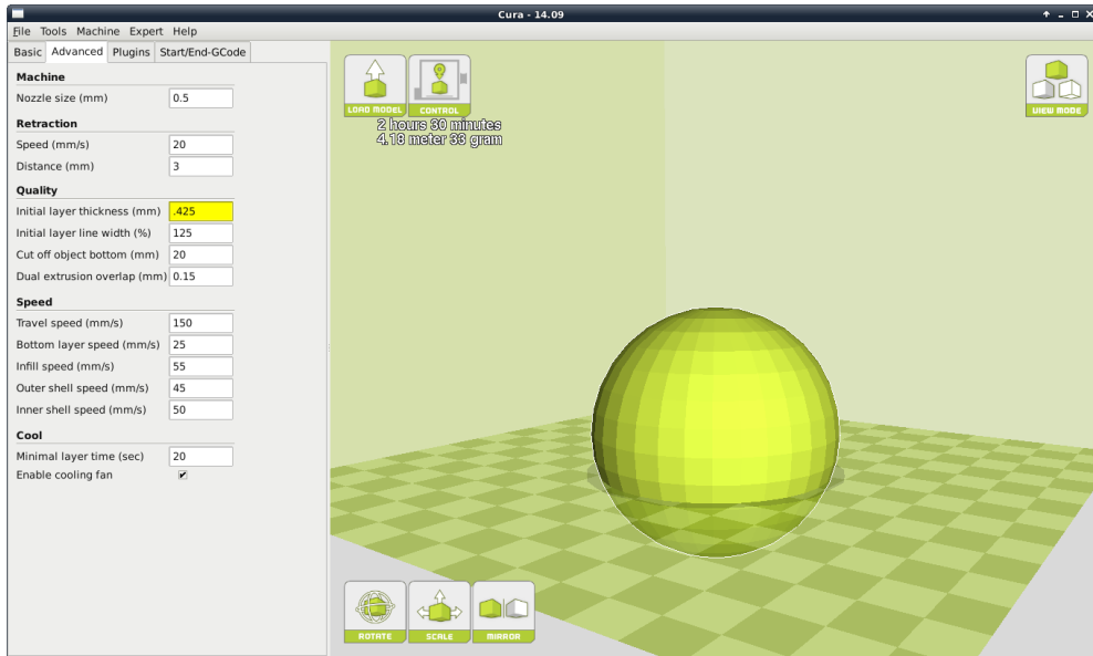
Figure 1.16: Cutoff Example
